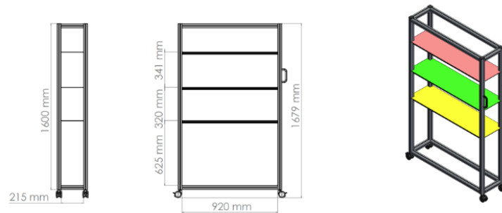
Figure 3: Shelf Dimensions
